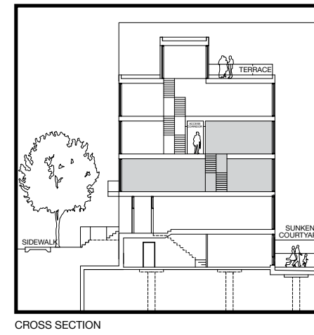
CROSS SECTION
